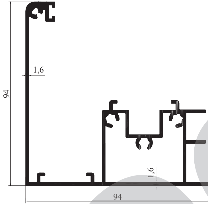
M 9510 - 1,891 kg/m
