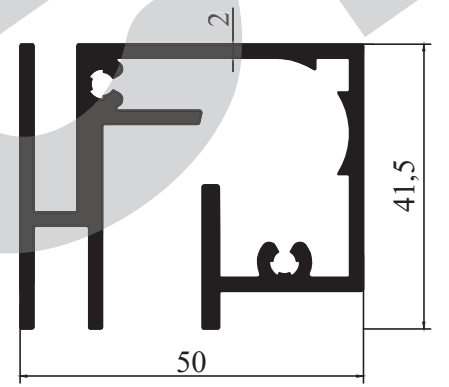
M 2475 - 1,420 kg/m
