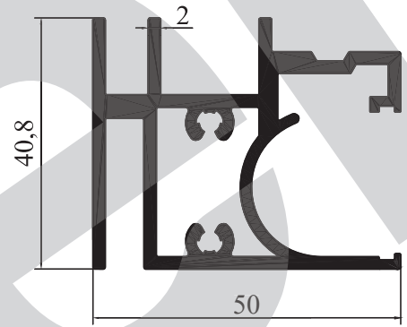
M 9512 - 1,401 kg/m
