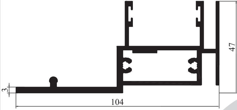
M 2476 - 1,873 kg/m
