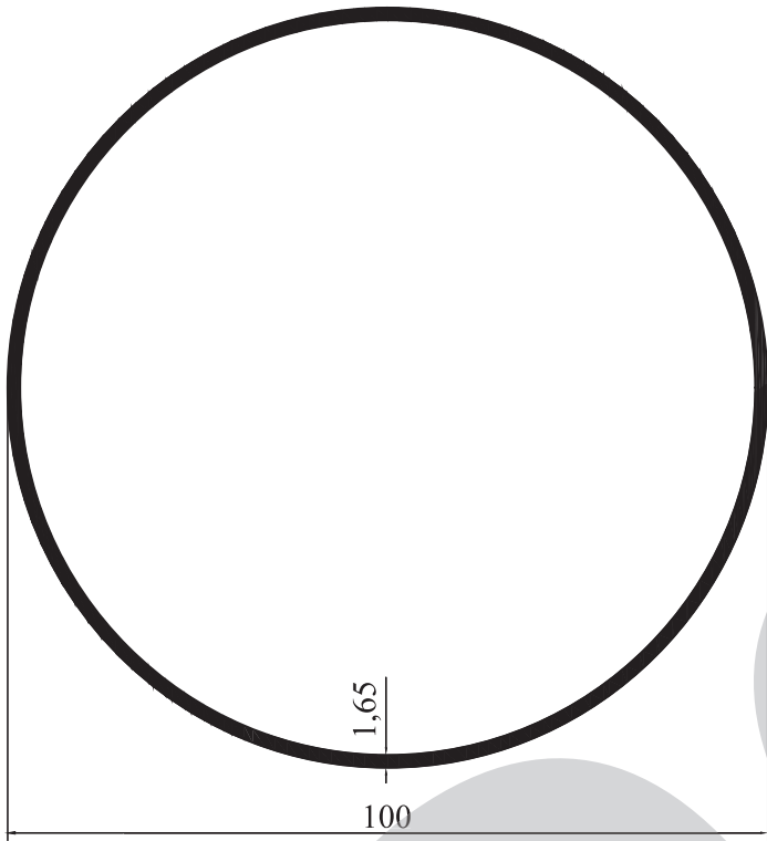
M 9525 - 1,381 kg/m
